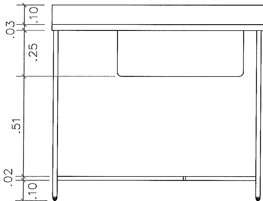
VISTA FRONTAL
